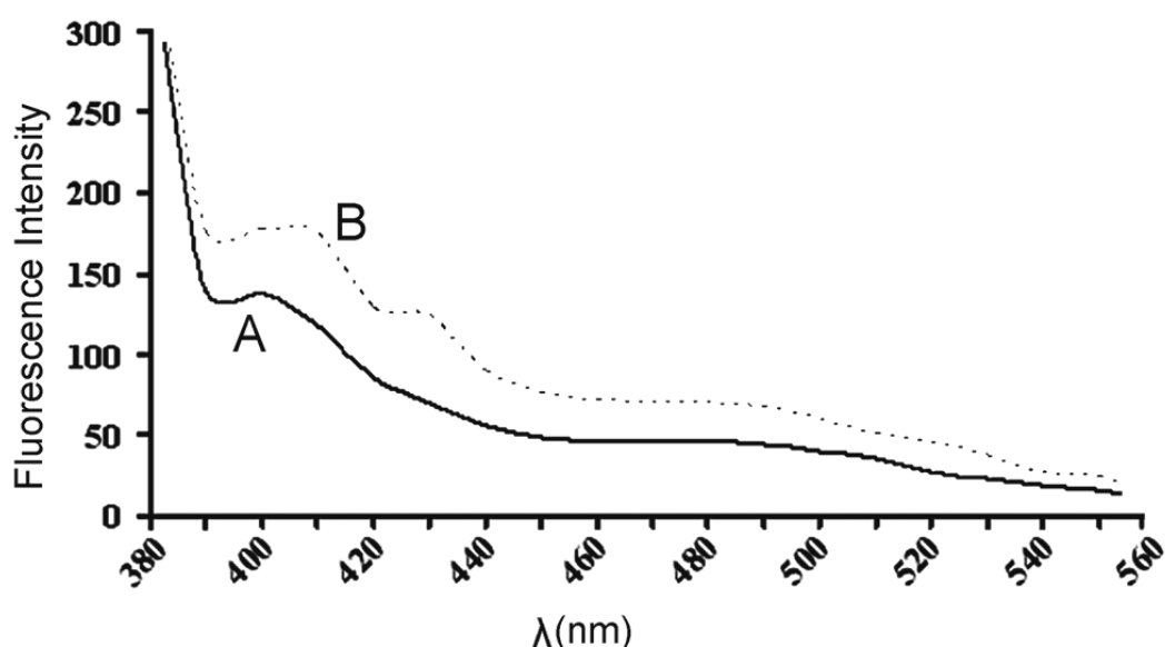
Figure 3: Fluorescence emission spectra for the reaction of nitrite with 2,3-diaminophthalene. In the emission spectra the curves A and B were, respectively: fungal filtrate and fungal filtrate and 0.1% \text{KNO}_3 solution. The maximum excitation wavelength was at 375 nm.
