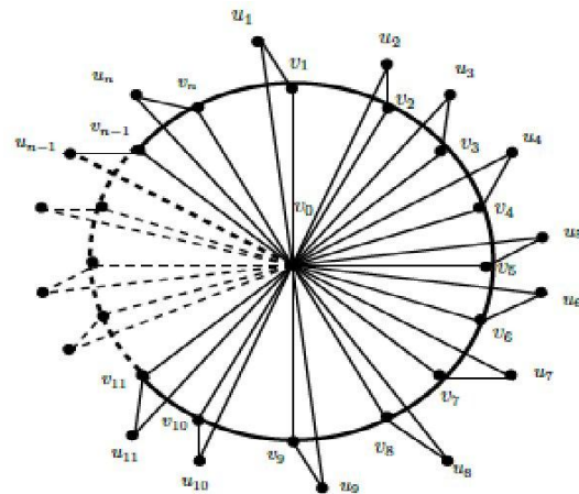
Figure 4. Flower graph Fl_n
