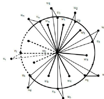
Figure 5. Sunflower graph Sf_n
