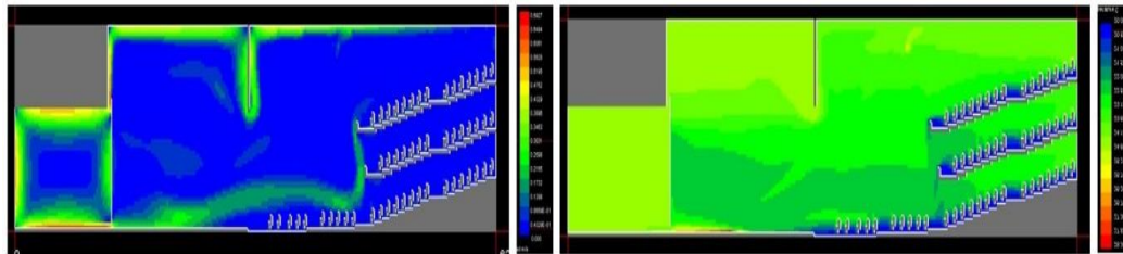
Figure 6. Case 3: when show is on and stage supply fans are off, simulation results
