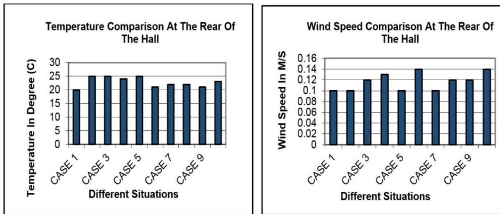
Figure 17. Temperature and wind speed comparison on Rear area
