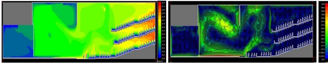
Figure 7. Case 4: When show is on and the stage supply of air is on, simulation results, source: Author
