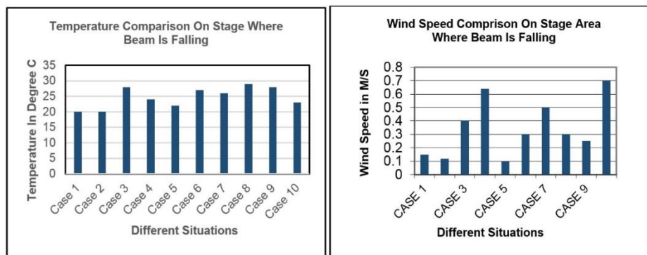
Figure 14. Temperature and wind speed comparison on stage area
