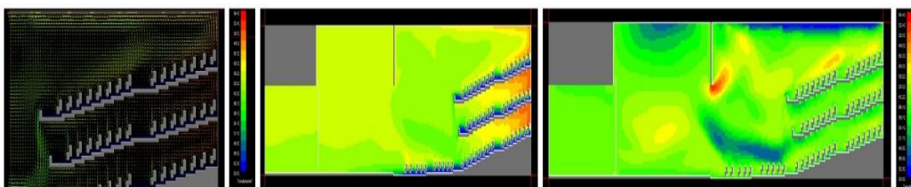
Figure 8. Case 5: when beam light is off during interval, simulation results
