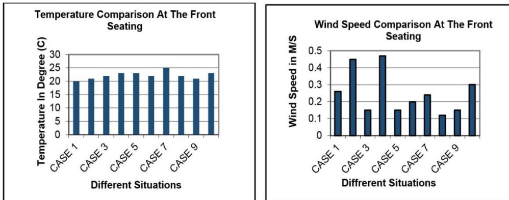
Figure 15. Temperature and wind speed comparison on front area
