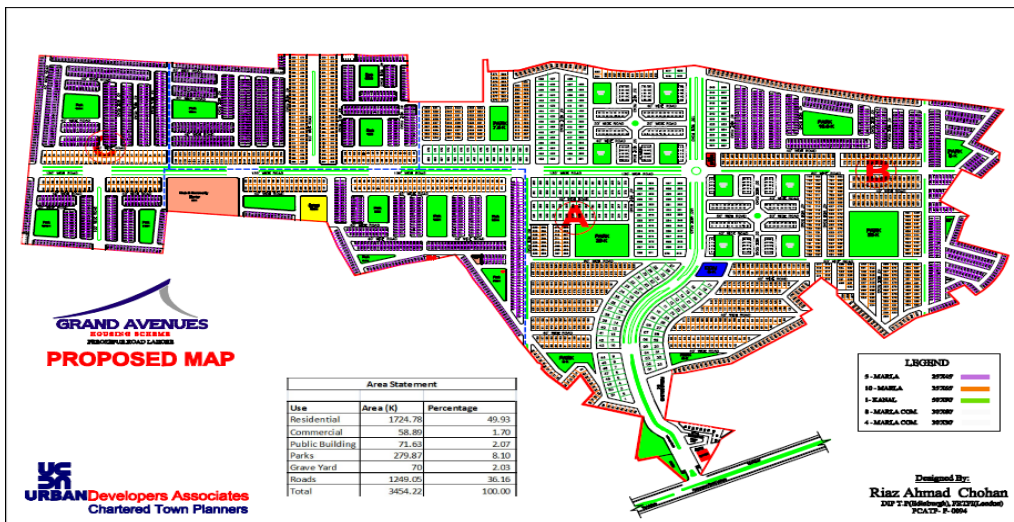
Figure 3. Master Plan of Grand Avenue Housing Scheme, Lahore
